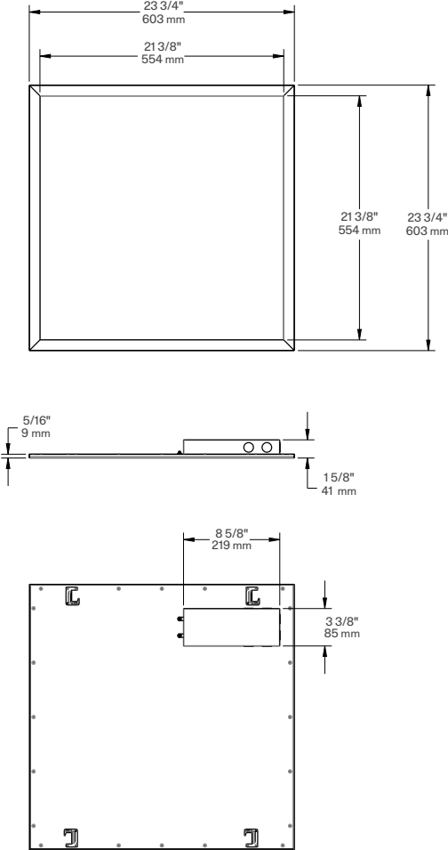
EZPAN® FA 2X2 Weight: 7.1 lbs.
