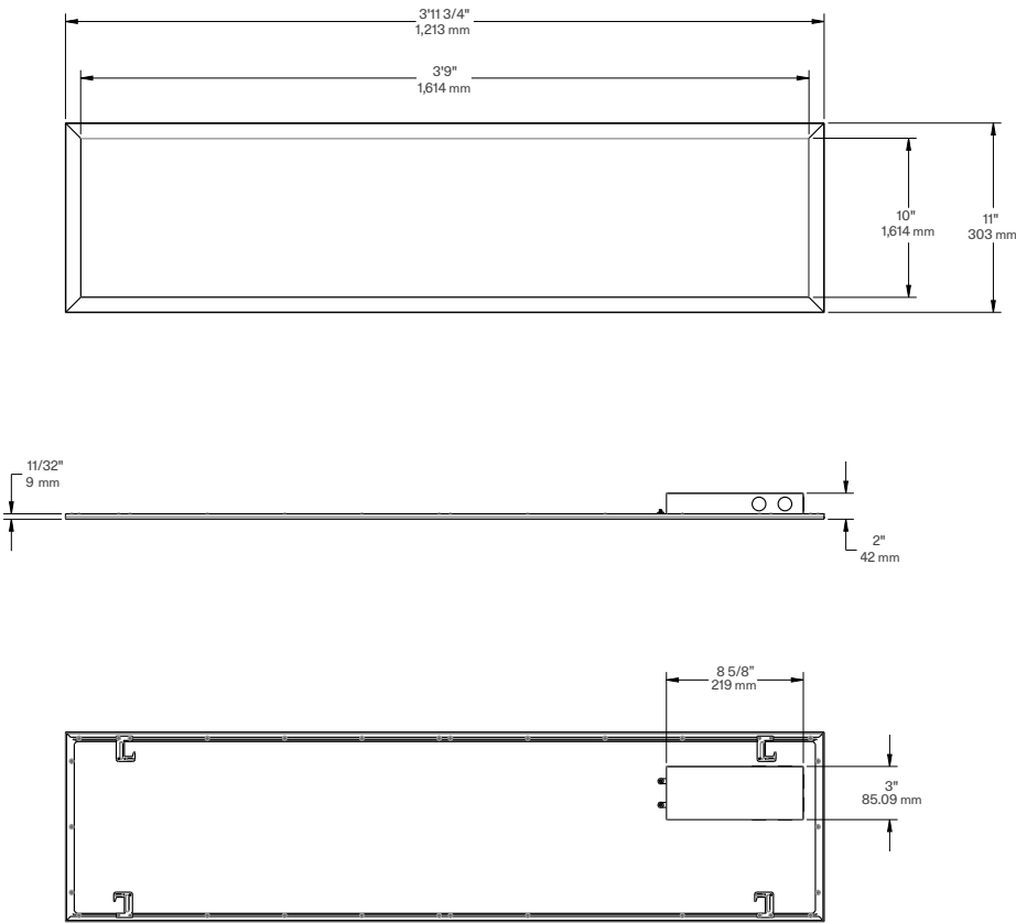
EZPAN® FA 1X4 Weight: 7.1 lbs.
