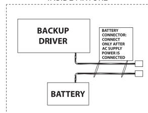
INSIDE FIXTURE
