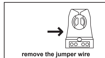
Fig:2 - External shunted Lampholder
